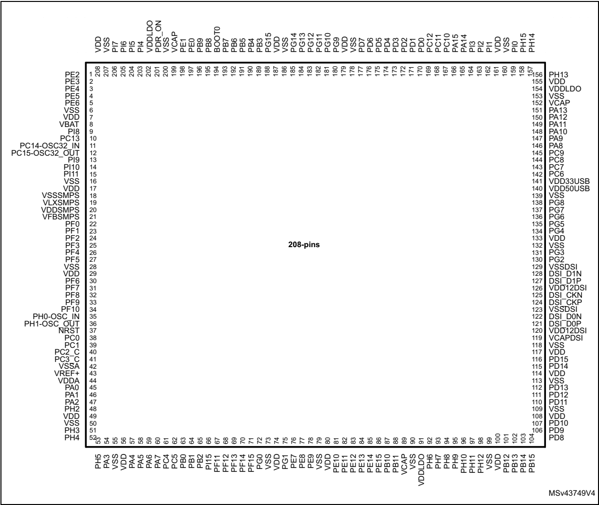
Figure 9. LQFP208 pinout
