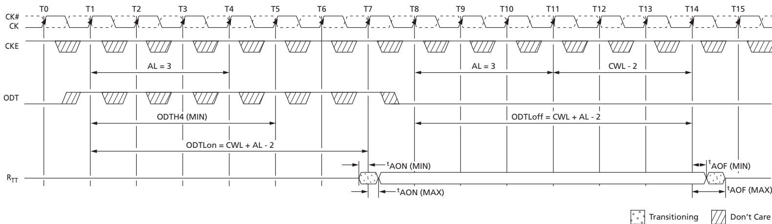
Figure 116: Synchronous ODT
