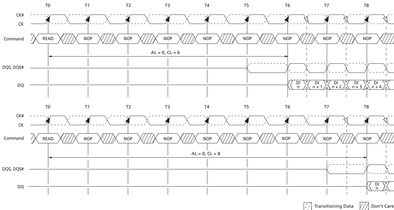
Figure 55: READ Latency
