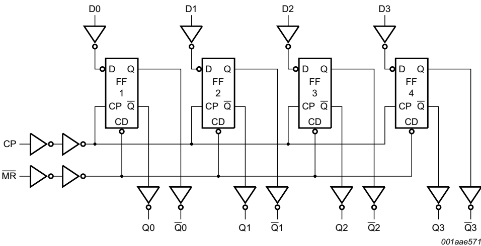
Fig 2. Logic diagram
