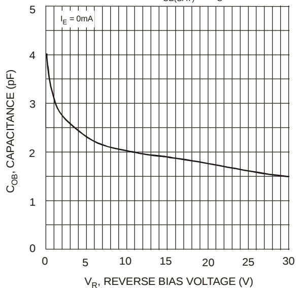
Fig. 4 Output Capacitance
