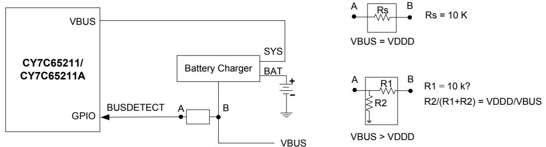
Figure 10. 9 V Tolerant
