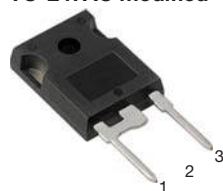
Base cathode 2 Cathode 1 Anode 3 VS-40EPS16PbF VS-40EPS16-M3
