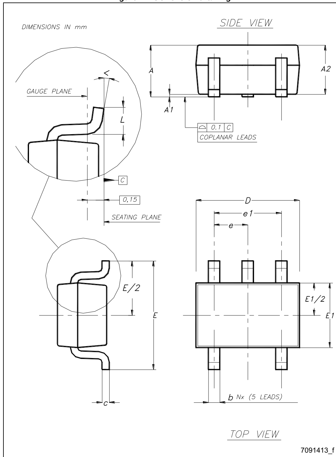
Figure 17. SOT323-5L drawing
