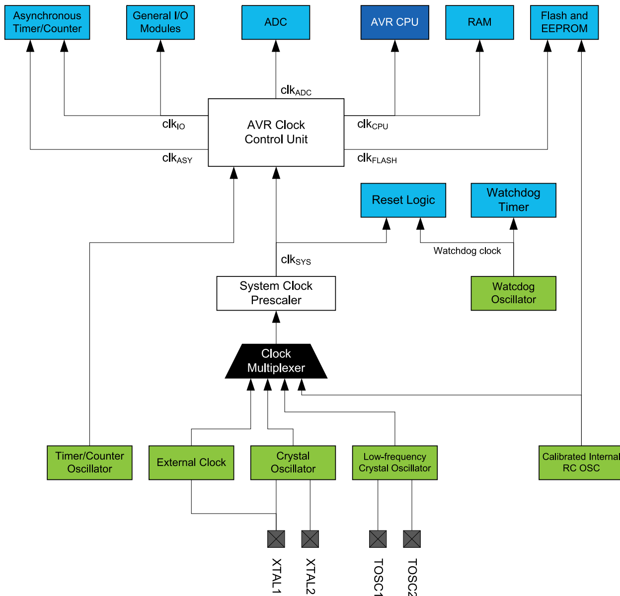
Figure 13-1. Clock Distribution
