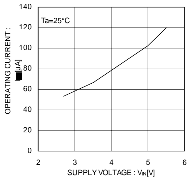
Figure 3. Operating current EN Enable
