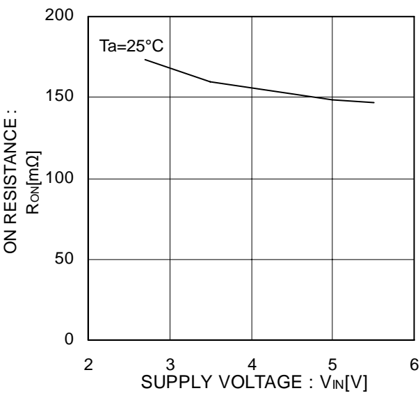
Figure 9. ON resistance
