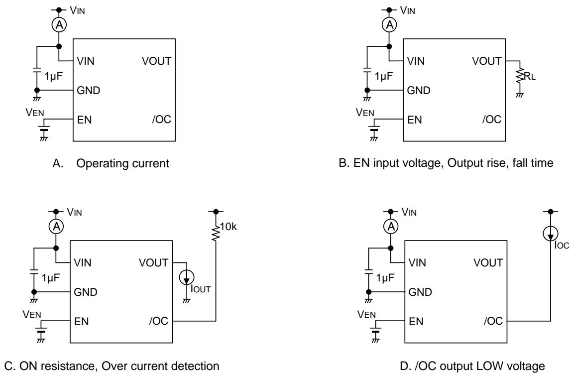
Figure 1. Measurement circuit
