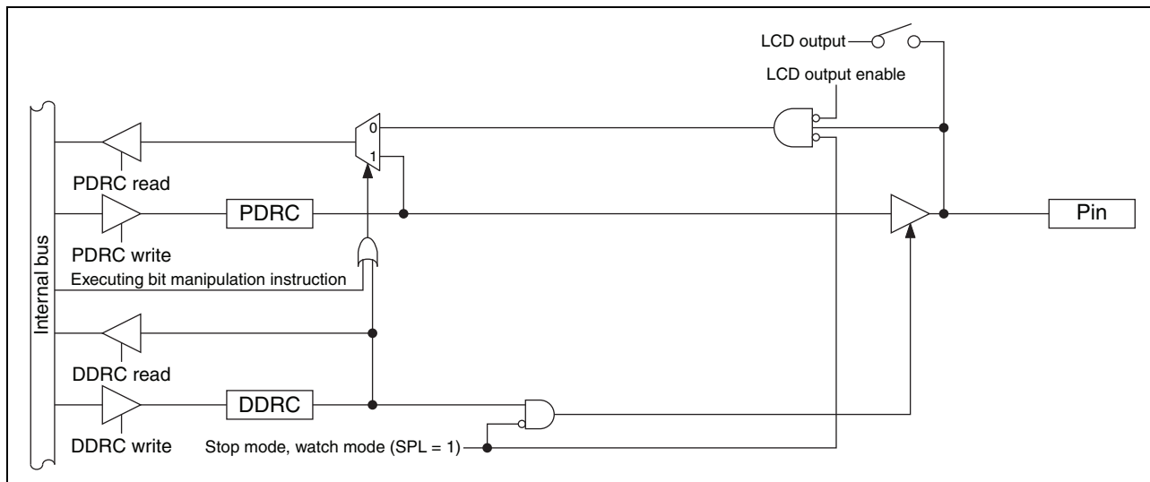
• Block diagram of PC0/SEG02, PC1/SEG03, PC2/SEG04, PC3/SEG05, PC4/SEG06, PC5/SEG07, PC6/SEG08 and PC7/SEG09
