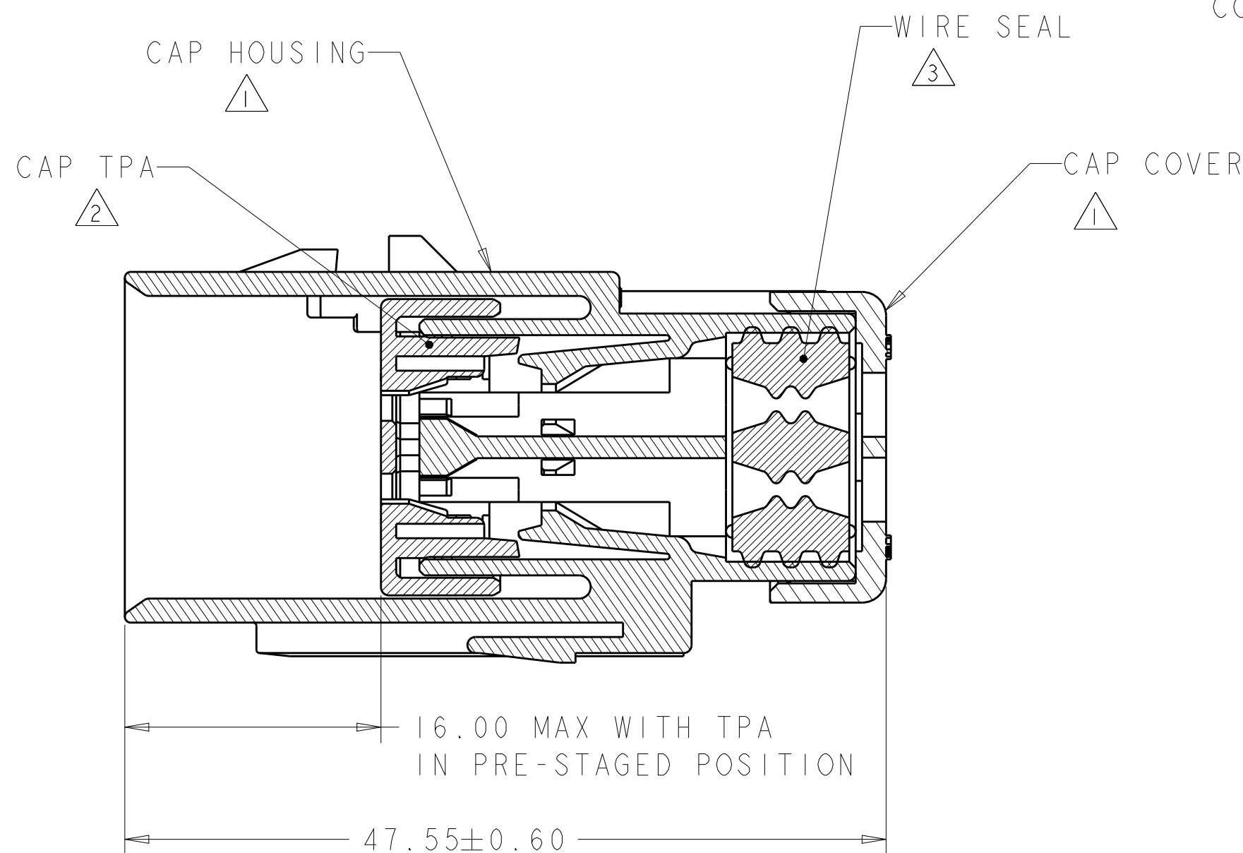
SECTION A-A OPEN POSITION
