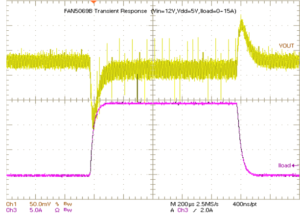
Figure 6. PWM Load Transient (0 to 15A)
