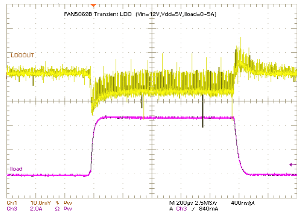
Figure 8. LDO Load Transient (0 to 5A)
