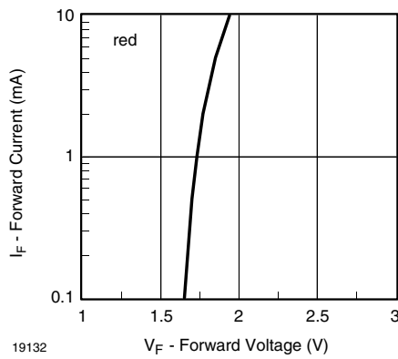
19132 Figure 14. Forward Current vs. Forward Voltage
