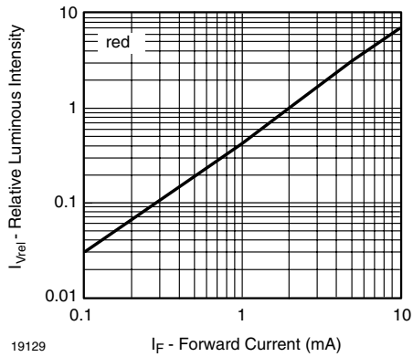
19129 Figure 13. Relative Luminous Intensity vs. Forward Current
