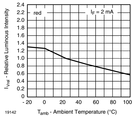
19142 Figure 17. Relative Luminous Intensity vs. Amb. Temperature
