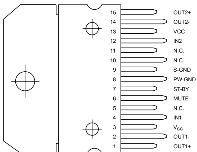
Figure 2. Pin connection (top view)
