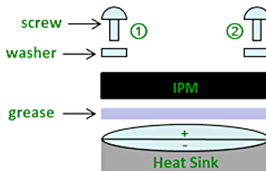
Figure 7. Mount HIC on a Heat Sink
