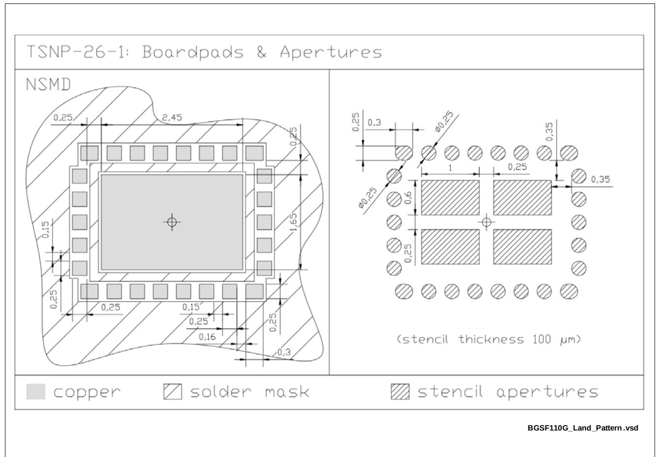
Figure 4 Land pattern
