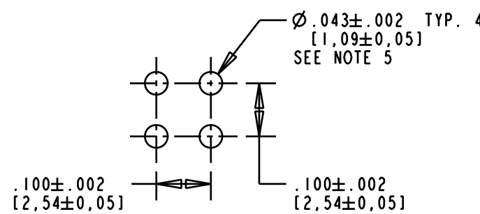
P.C. BOARD HOLE PATTERN
