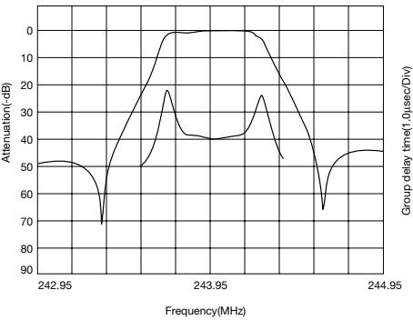
PAFC243B Pass Band Characteristics
