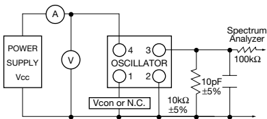
Test Circuit 2 (Harmonics and Frequency)
