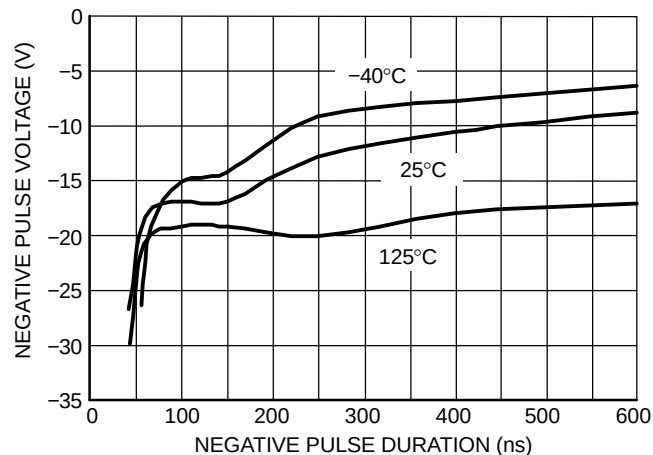
Figure 52. NCP5106B, Negative Voltage Safe Operating Area on the Bridge Pin
