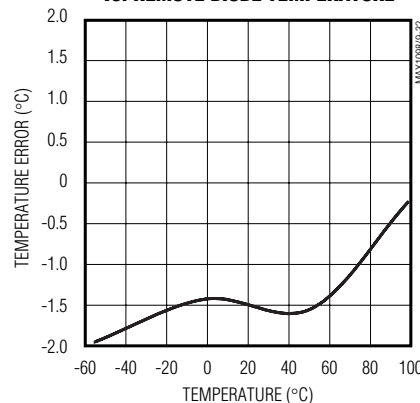
MAX1099 TEMPERATURE ERROR vs. REMOTE DIODE TEMPERATURE
