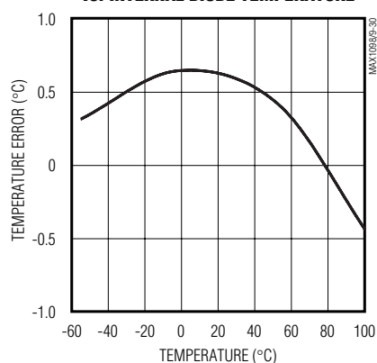
MAX1099 TEMPERATURE ERROR vs. INTERNAL DIODE TEMPERATURE
