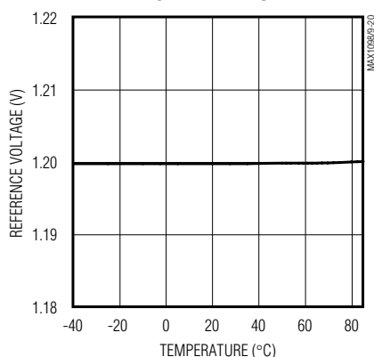
MAX1099 INTERNAL REFERENCE VOLTAGE vs. TEMPERATURE
