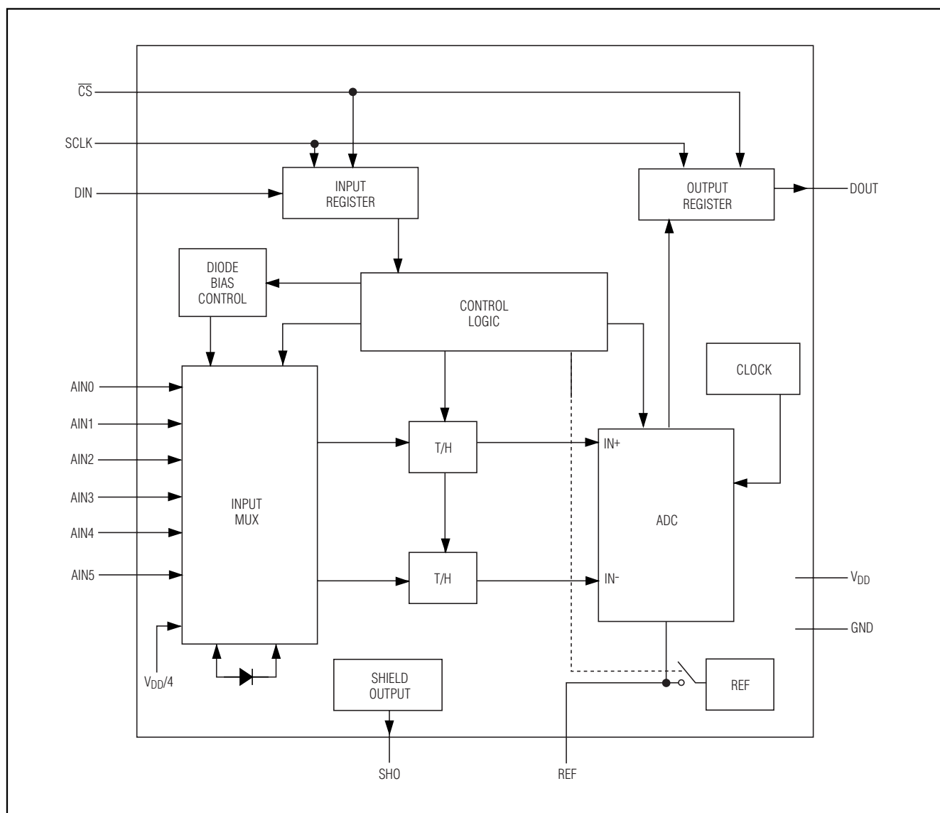
Figure 1. MAX1098/MAX1099 Functional Diagram
