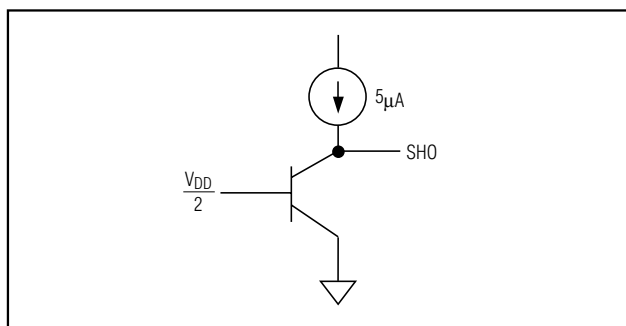
Figure 7. SHO Output Circuit
