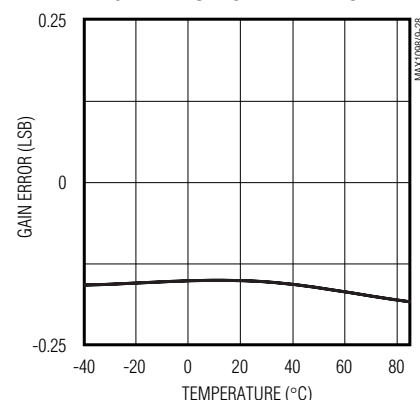
MAX1099 GAIN ERROR vs. TEMPERATURE
