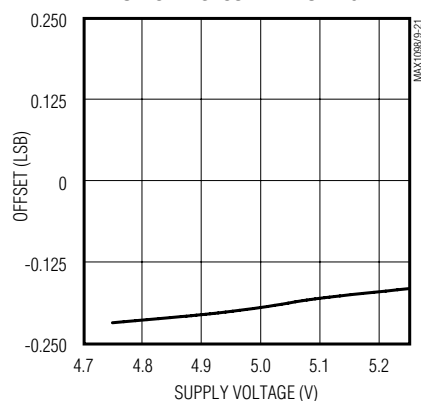
MAX1098 OFFSET vs. SUPPLY VOLTAGE
