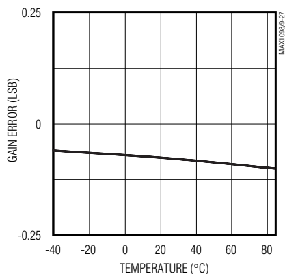
MAX1098 GAIN ERROR vs. TEMPERATURE
