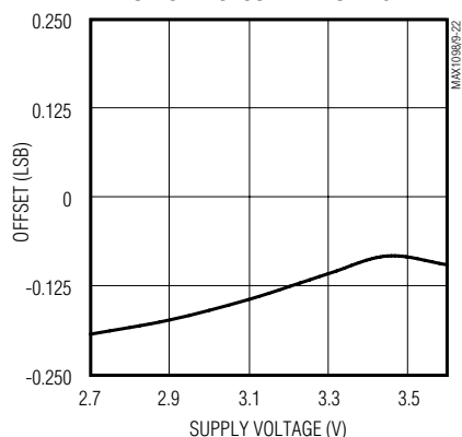
MAX1099 OFFSET vs. SUPPLY VOLTAGE
