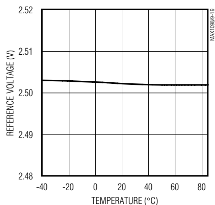
MAX1098 INTERNAL REFERENCE VOLTAGE vs. TEMPERATURE
