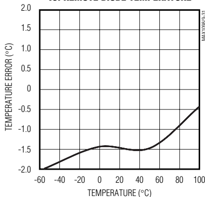
MAX1098 TEMPERATURE ERROR vs. REMOTE DIODE TEMPERATURE
