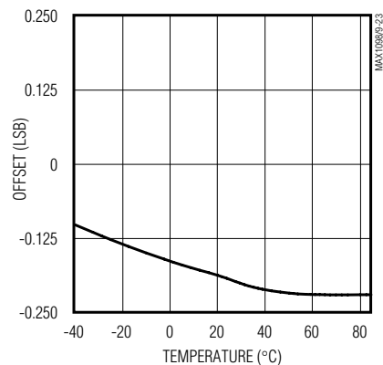
MAX1098 OFFSET vs. TEMPERATURE
