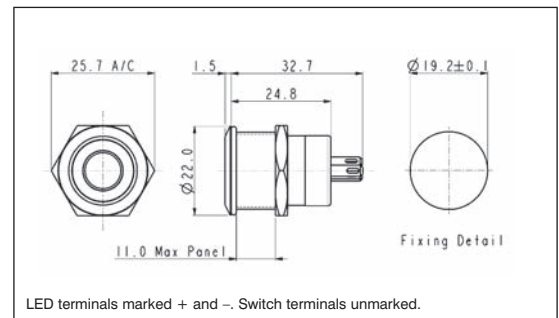
LED terminals marked + and -. Switch terminals unmarked.
