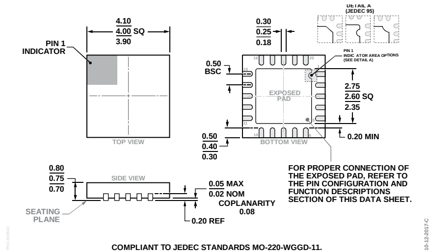
Figure 54. 20-Lead Lead Frame Chip Scale Package [LFCSP] 4 mm × 4 mm Body and 0.75 mm Package Height (CP-20-8) Dimensions shown in millimeters
