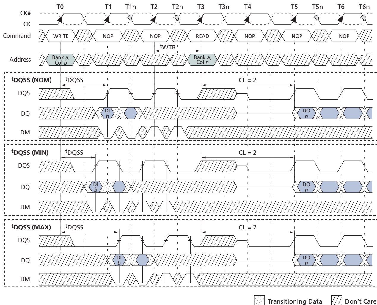
Figure 42: WRITE-to-READ – Interrupting
