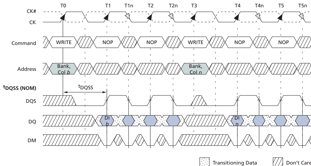
Figure 39: Nonconsecutive WRITE-to-WRITE
