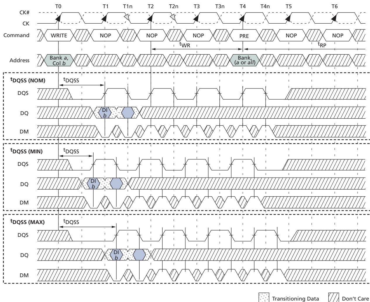
Figure 45: WRITE-to-PRECHARGE – Interrupting
