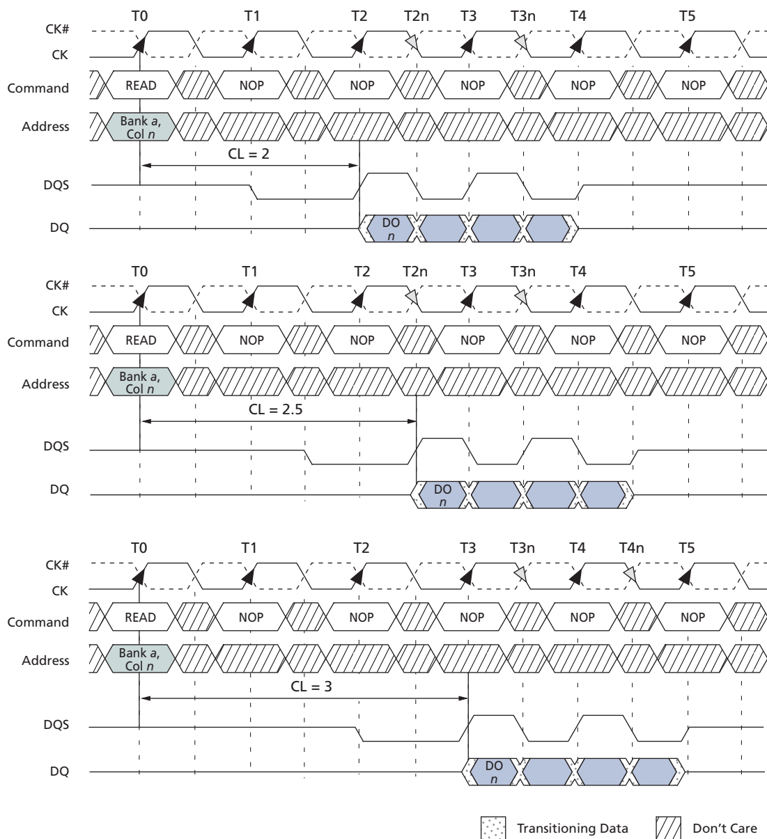
Figure 26: READ Burst
