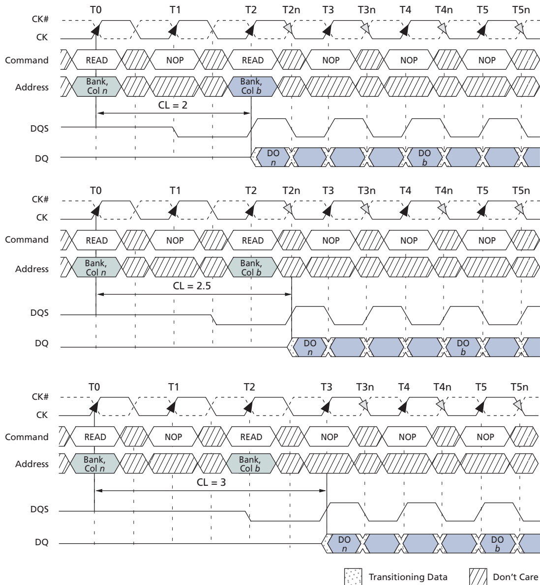
Figure 27: Consecutive READ Bursts
