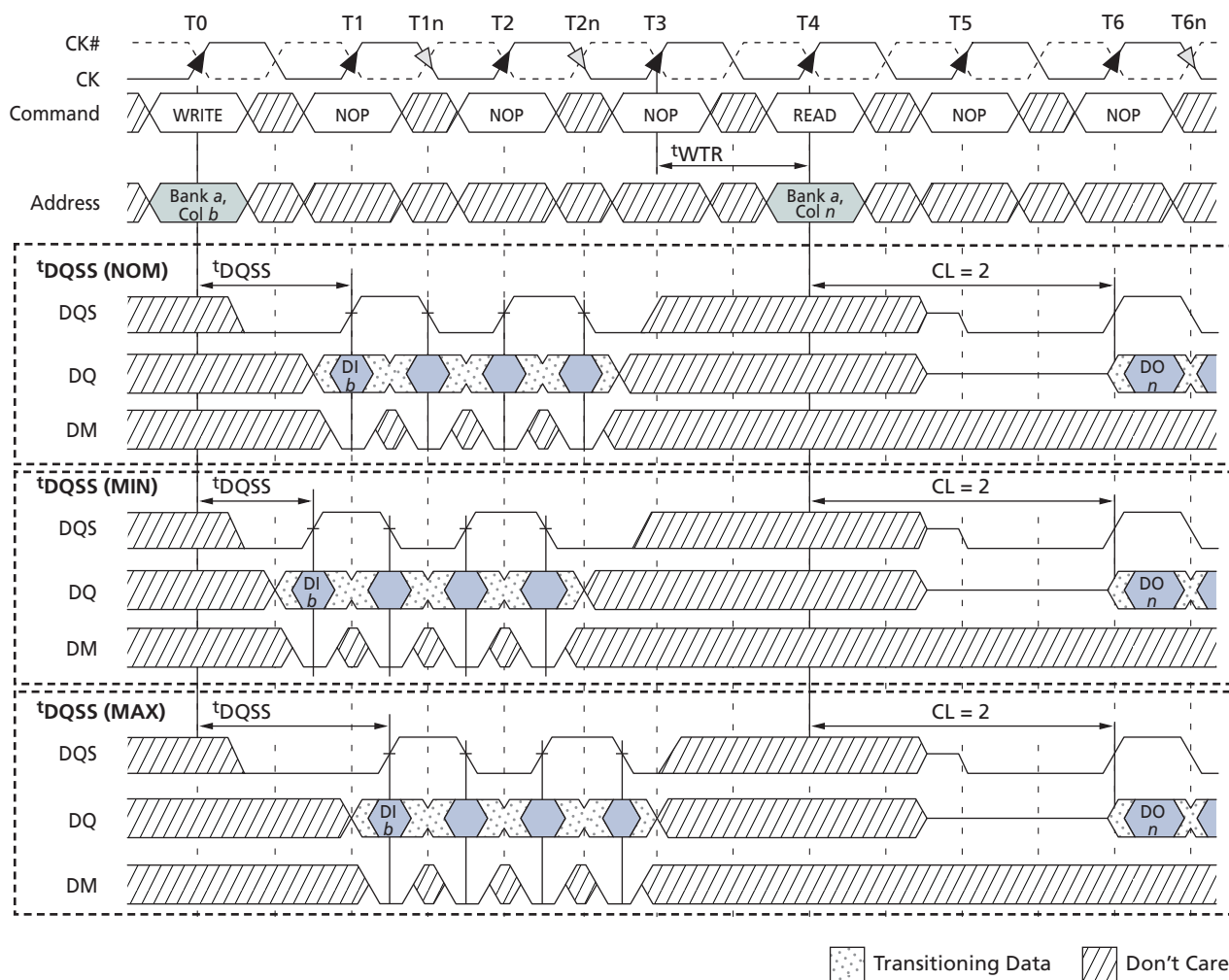
Figure 41: WRITE-to-READ – Uninterrupting
