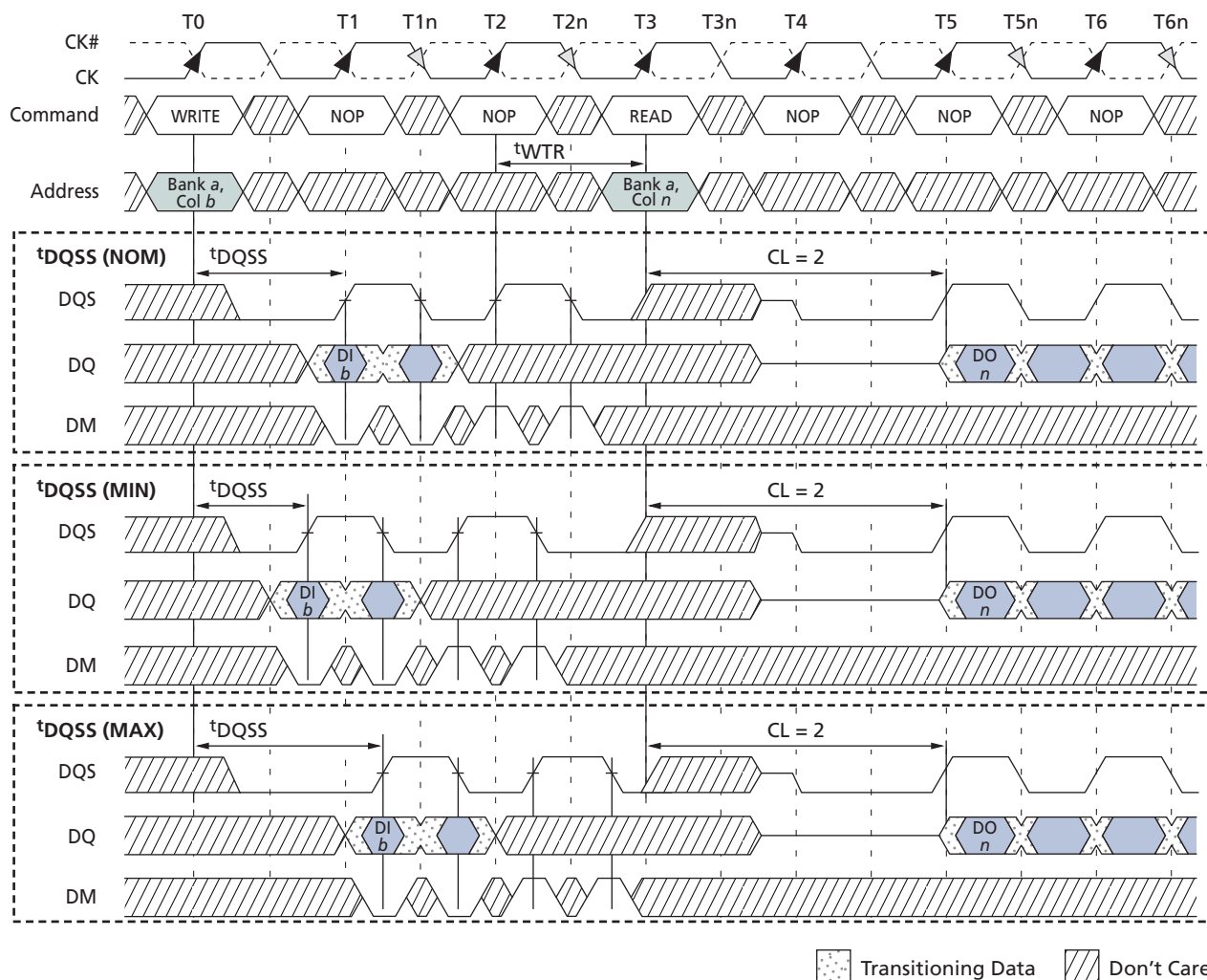
Figure 42: WRITE-to-READ – Interrupting
