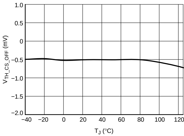
Figure 19. CS Turn-off Threshold
