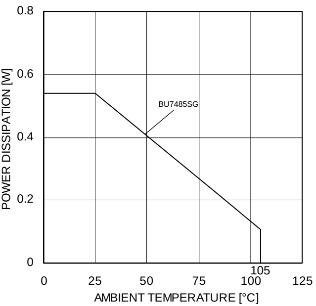
Figure 3. Derating curve
