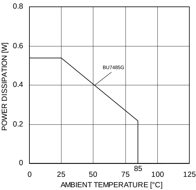
Figure 2. Derating curve
