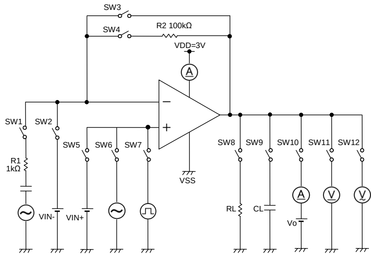
Figure 72. Test circuit 2
