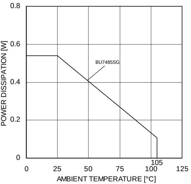
Figure 3. Derating curve
