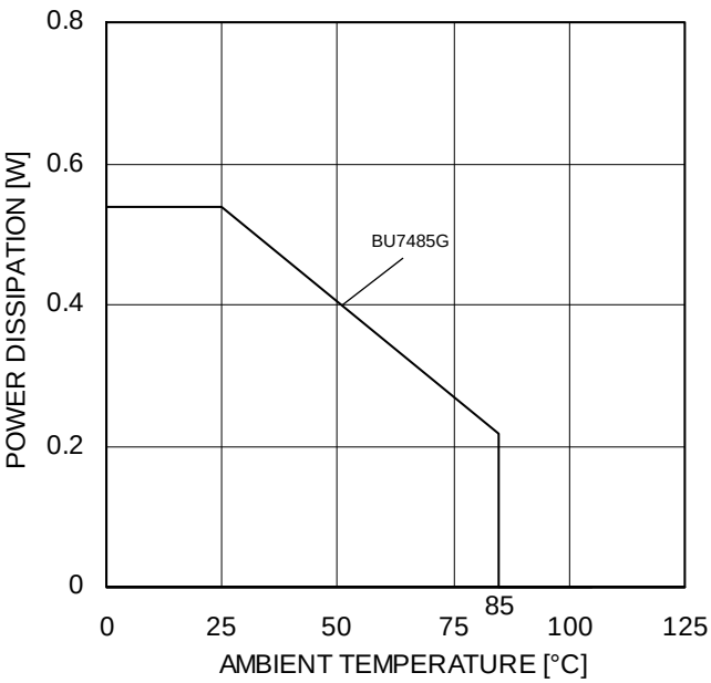
Figure 2. Derating curve
