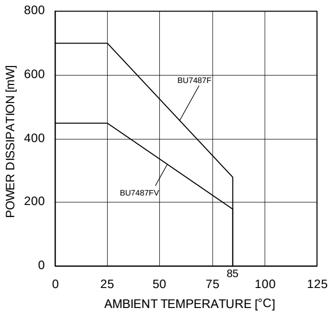
Figure 48. Derating curve
