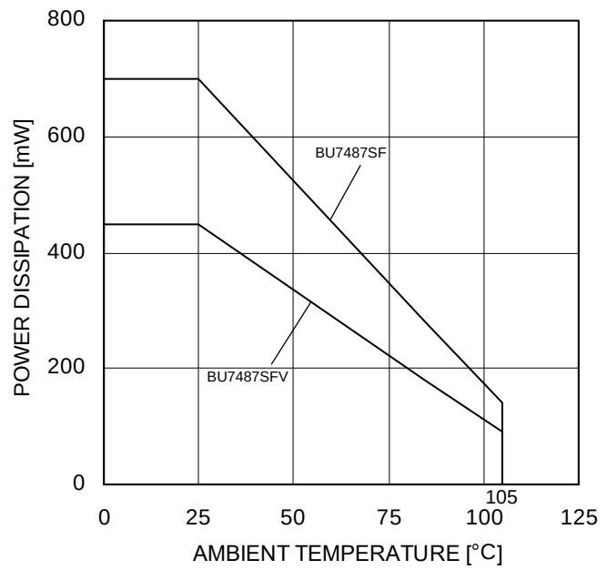
Figure 49. Derating curve
