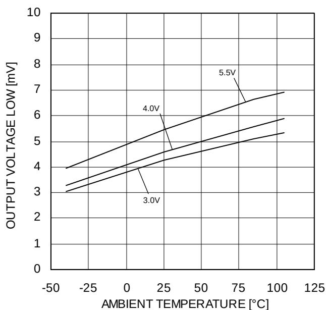
Figure 32. Maximum Output Voltage Low – Ambient Temperature (RL=10kΩ)
