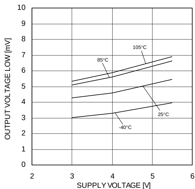
Figure 31. Maximum Output Voltage Low – Supply Voltage (RL=10kΩ)
