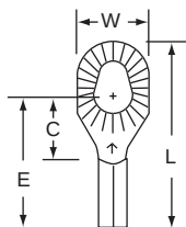
11-610 Stud Size Wire Range 6, 8, 10 22-18
