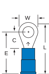
12-10-P Stud Size 10 Wire Range 16-14
