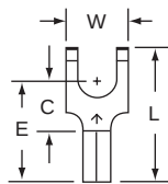
BS-21-10 Stud Size 10 Wire Range 22-18
