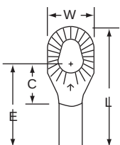
12-610-W Stud Size Wire Range 6, 8, 10 16-14
