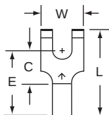
BS-22-6-W Stud Size 6 Wire Range 16-14
