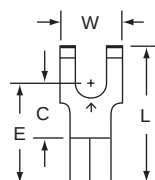
BS-23-8 Stud Size 8 Wire Range 12-10
