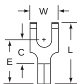
BS-21-6 Stud Size 6 Wire Range 22-18
