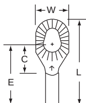
11-610-W Stud Size Wire Range 6, 8, 10 22-18
