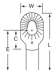
13-610-W Stud Size Wire Range 6, 8, 10 12-10
