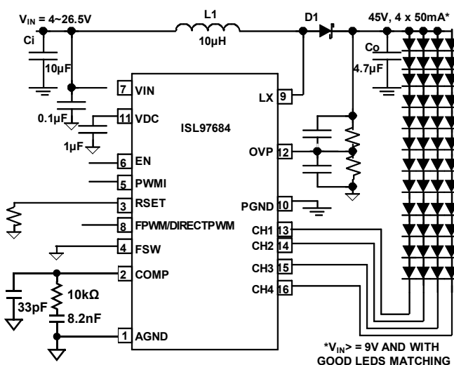
FIGURE 1A. DIRECT PWM DIMMING
