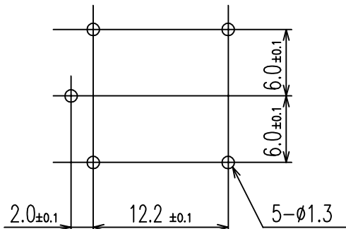
4.DRILLING DIAGRAM(BOTTOM VIEW)
