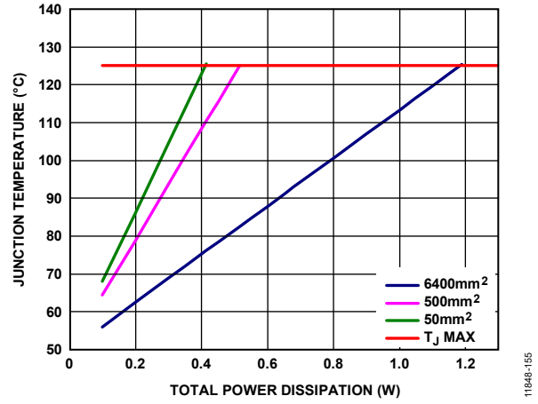
Figure 56. SOIC, T A = 50°C
