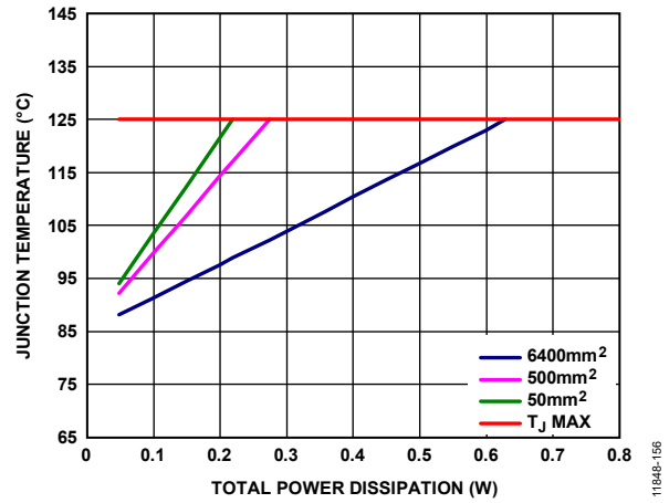
Figure 57. SOIC, T A = 85°C
