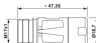
Dimensional drawing
