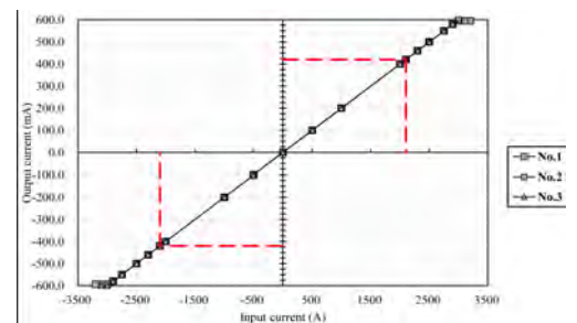
Saturation Characteristics
