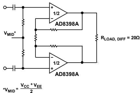
Figure 8. Typical Differential Application Circuit R_{\text{LOAD, DIFF}} = 20\ \Omega
