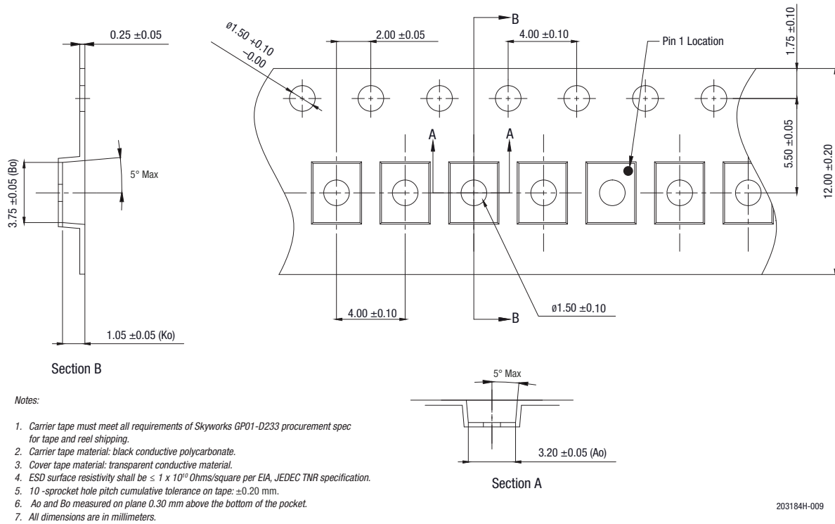
Figure 9. SKY66110-11 Tape and Reel Dimensions
