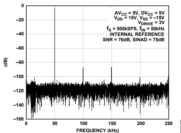
Figure 5. AD7367-5 FFT
