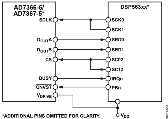
Figure 32. Interfacing the AD7366-5/AD7367-5 to the DSP563xx
