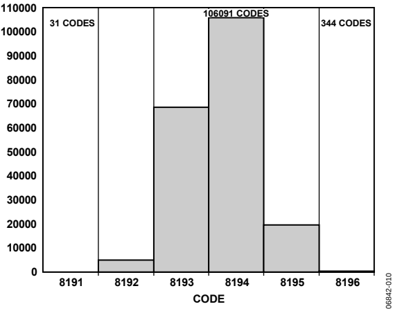
Figure 10. Histogram of Codes for 200k Samples
