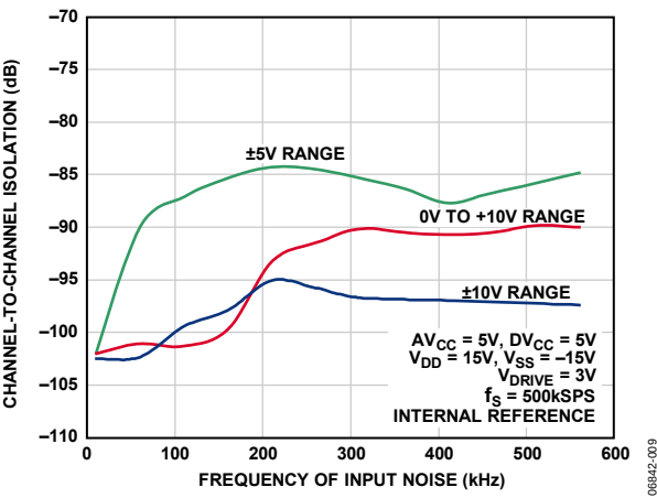
Figure 9. Channel-to-Channel Isolation
