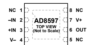
Figure 1. AD8597 8-Lead SOIC (R-8)
