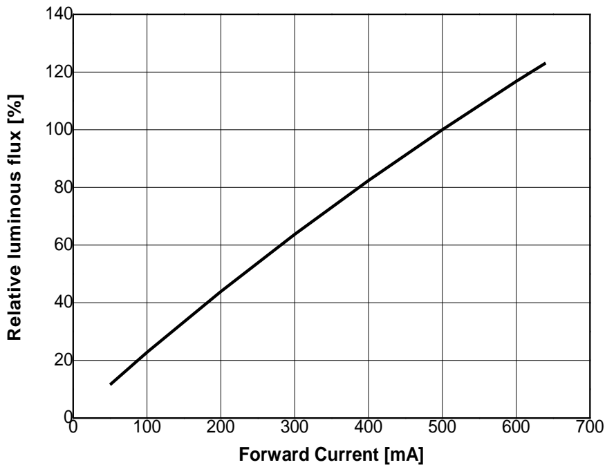
Fig 4. Forward Current vs. Relative Luminous Flux, Ta=25°C
