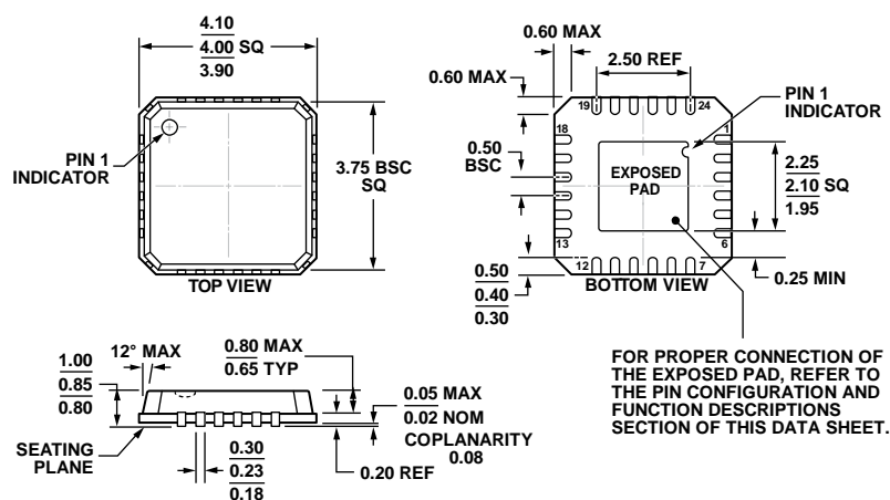
Figure 44. 24-Lead Lead Frame Chip Scale Package [LFCSP_VQ]
