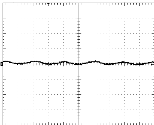
Fig.1.8V-9: Input reflected ripple current, I_s (5mA/div), measured through 10µH at the source at full rated load current and V_{in}=48V . Time scale: 1µs/div.
