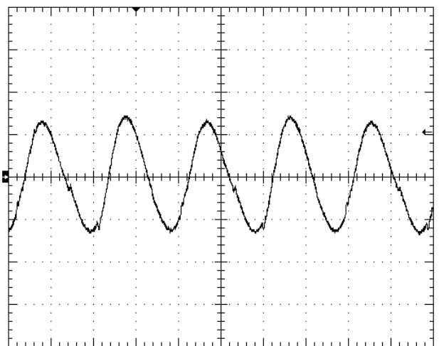
Fig.1.8V-10: Input reflected ripple current, I_c (100mA/div), measured through 10µH at the source at full rated load current and V_{in}=48V . Time scale: 1µs/div.
