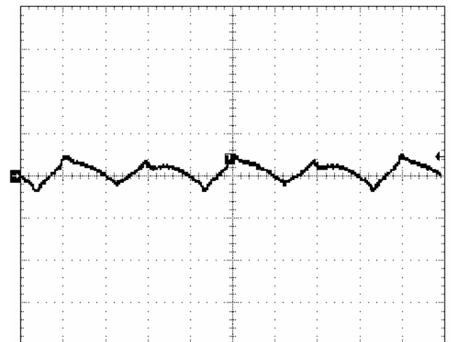
Fig.1.8V-7: Output voltage ripple (50mV/div) at full rated load current into a resistive load with Co=10 \mu F tantalum + 1 \mu F ceramic and Vin=48V. Time scale: 1 \mu s/div
