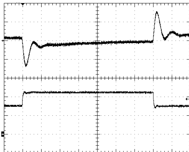
Fig.1.8V-6: Output voltage response to load current step-change (15 \leftrightarrow 22.5A) at Vin=48V. Top trace: Output voltage (100mV/div). Bottom trace: load current (10A/div). Current slew rate: 5A/ \mu s. Co=470 \mu F os-con + 10 \mu F tantalum + 1 \mu F ceramic. Time scale: 100 \mu s/div
