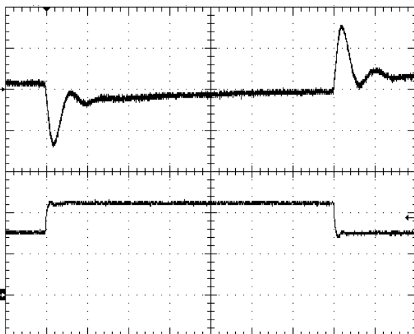
Fig.1.8V-6: Output voltage response to load current step-change (15⇌22.5A) at Vin=48V. Top trace: Output voltage (100mV/div). Bottom trace: load current (10A/div). Current slew rate: 5A/µs. Co=470µF os-con + 10µF tantalum + 1µF ceramic. Time scale: 100µs/div
