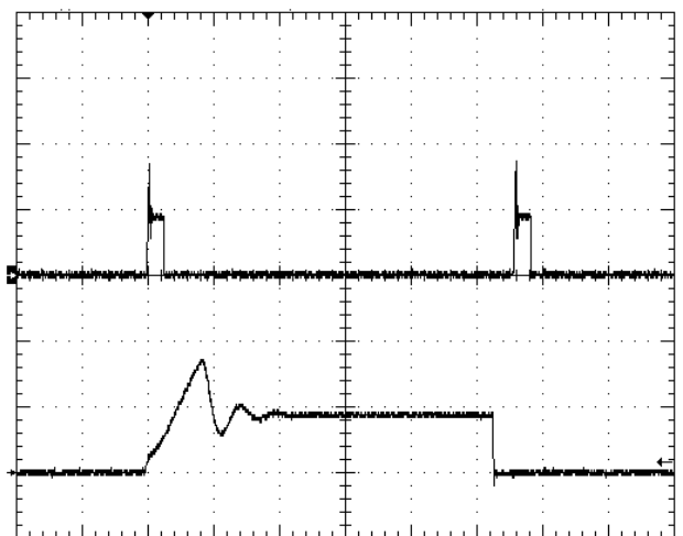
Fig.1.8V-12: Load current (top trace, 50A/div, 20ms/div) into a 10mΩ short circuit during restart, at V_{in} = 48V . Bottom trace (50A/div, 5ms/div) is an expansion of the top trace.
