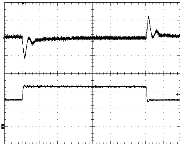
Fig.2.5V-6: Output voltage response to load current step-change (15 \leftrightarrow 22.5A) at Vin=48V. Top trace: Output voltage (100mV/div). Bottom trace: load current (10A/div). Current slew rate: 5A/ \mu s. Co=470 \mu F os-con + 10 \mu F tantalum + 1 \mu F ceramic. Time scale: 100 \mu s/div
