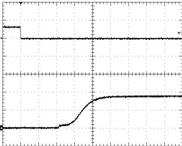
Fig.1.8V-4: Turn-on transient at full rated load current (resistive) with 10µF tantalum + 1µF ceramic capacitor at Vin=48V, triggered via ON/OFF pin. Top trace: ON/OFF signal (5V/div). Bottom trace: output voltage (1V/div). Time scale: 2ms/div
