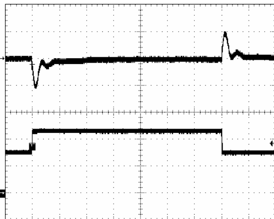
Fig.3.3V-6: Output voltage response to load current step-change (15A \leftrightarrow 22.5A) at Vin=48V. Top trace: Output voltage (100mV/div). Bottom trace: load current (10A/div). Current slew rate: 5A/ \mu s. Co=470 \mu F os-con + 10 \mu F tantalum + 1 \mu F ceramic. Time scale: 100 \mu s/div
