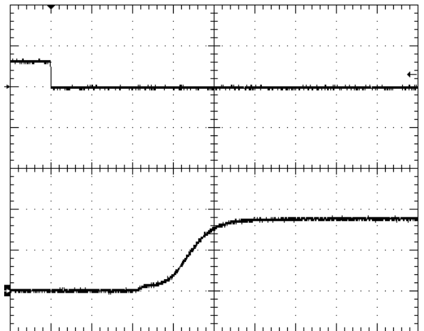
Fig.1.8V-5: Turn-on transient at full rated load current (resistive) plus 20,000µF at Vin=48V, triggered via ON/OFF pin. Top trace: ON/OFF signal (5V/div). Bottom trace: output voltage (1V/div). Time scale: 2ms/div
