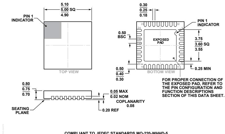
Figure 57. 32-Lead Lead Frame Chip Scale Package [LFCSP] 5 mm × 5 mm Body and 0.75 mm Package Height (CP-32-12) Dimensions shown in millimeters
