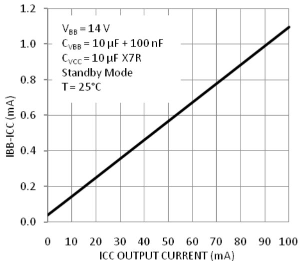
Figure 14. Ground Current vs. Output Current
