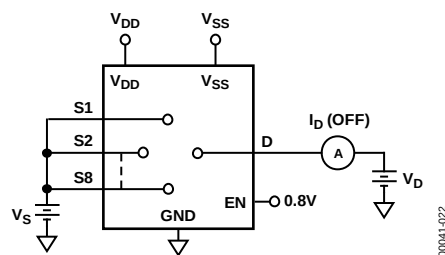
Figure 22. I_D (OFF)
