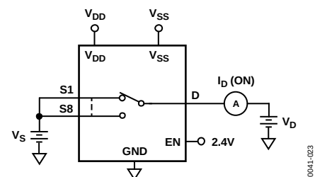
Figure 23. I_D (ON)
