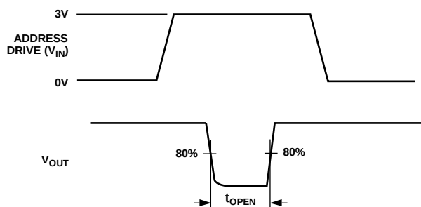
Figure 25. Break-Before-Make Delay, t_{OPEN}
