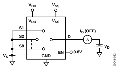
Figure 22. I_D (OFF)
