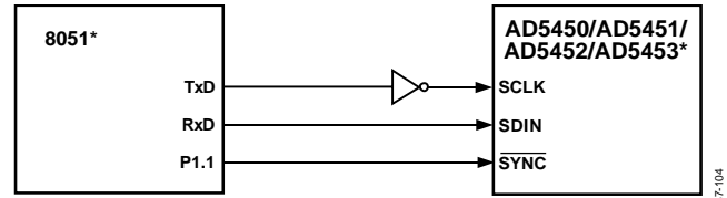
Figure 59. 80C51/80L51 to AD5450/AD5451/AD5452/AD5453 Interface
