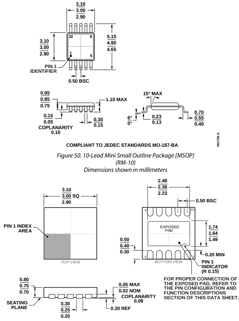
Figure 51. 10-Lead Lead Frame Chip Scale Package [LFCSP_WD] 3 mm × 3 mm Body, Very Very Thin, Dual Lead (CP-10-9) Dimensions shown in millimeters
